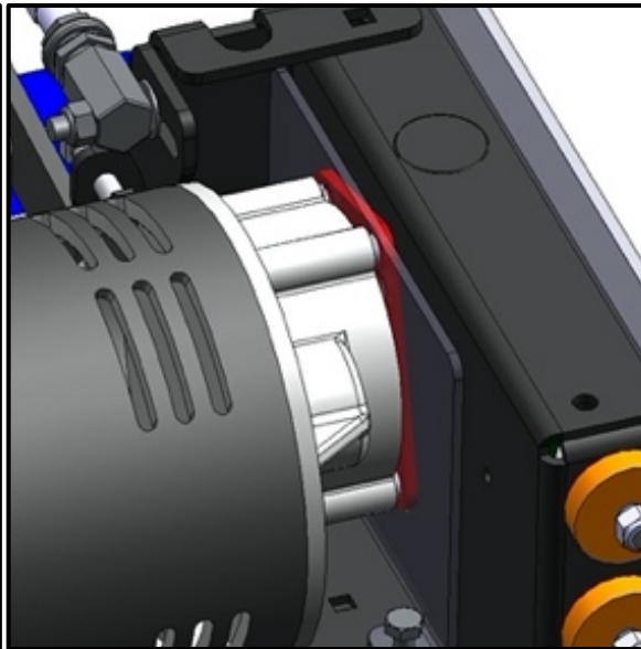
(New Spacer Plate in RED )
