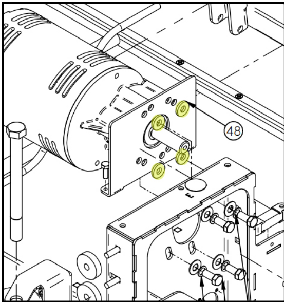
(Old Washers in YELLOW )
